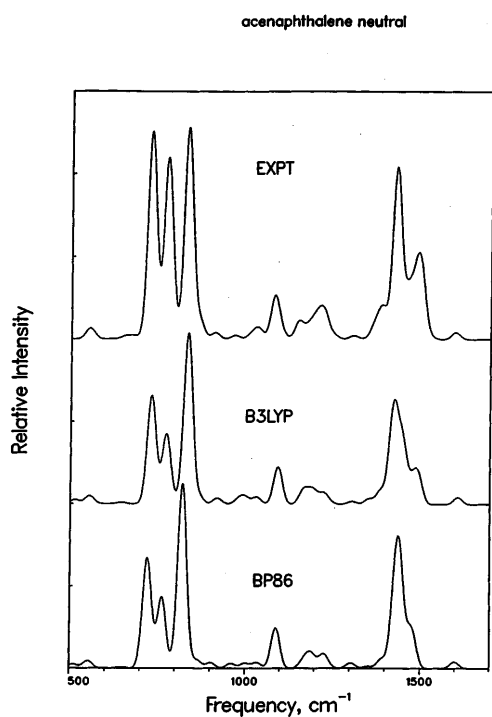
Fig. 2. The BP86, B3LYP, and experimental spectra of acenaphthalene. The full width at half-maximum ( FWHM ) is 30\text{ cm}^{-1}
