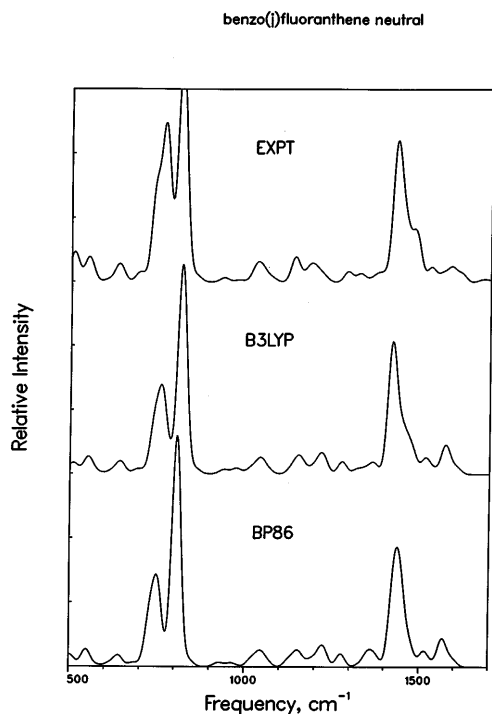
Fig. 6. The BP86, B3LYP, and experimental spectra of benzo[ j ]fluoranthene. The FWHM is 30 \text{cm}^{-1}
